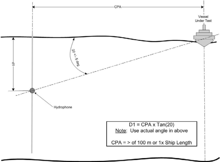
Figure 1 – Grades A and B hydrophone geometry.
