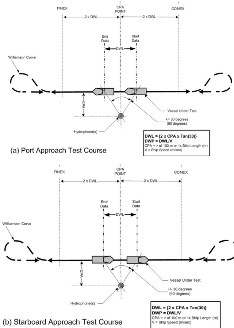
Figure 3 – Test course configuration, (a) port and (b) starboard approaches.
