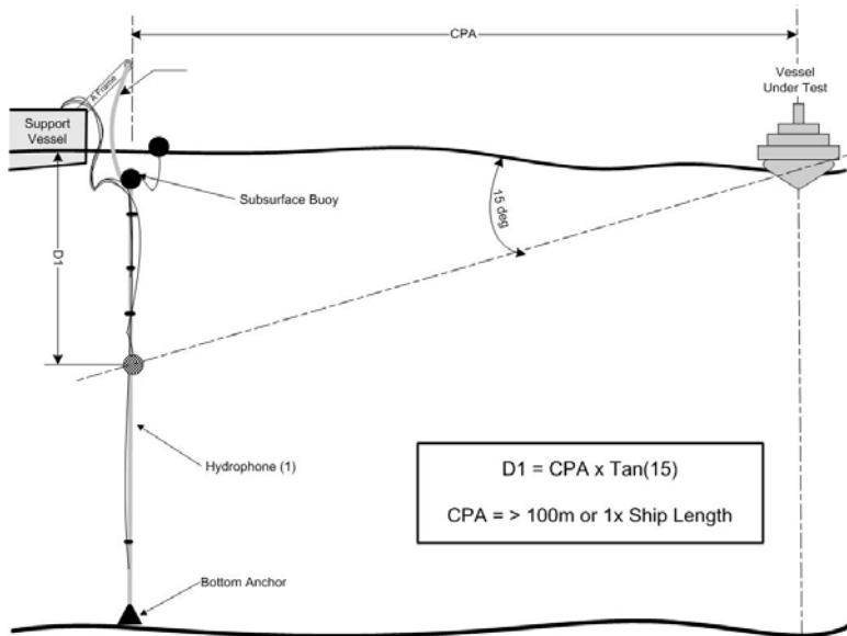
Figure 1 – Grades A and B Hydrophone Deployment Configuration.
