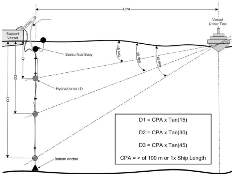
Figure 1 – Grades A and B Hydrophone Deployment Configuration.
