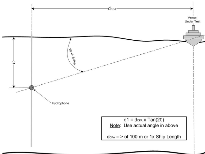
Figure 2 – Grade C hydrophone geometry.
